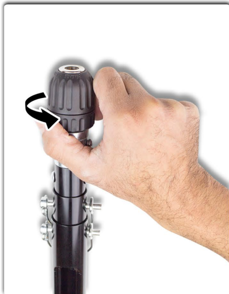
Step 3. Turn the top portion of the Keyless Chuck counter-clockwise to open the jaws
