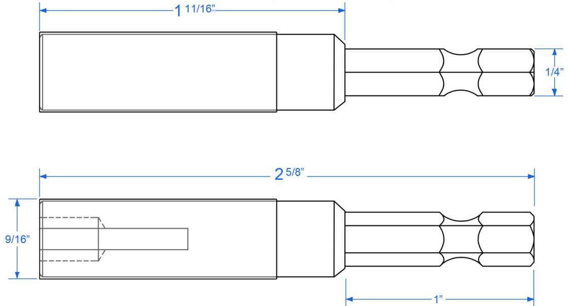
SIDE VIEW
